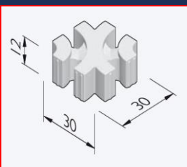
Geological Pattern
